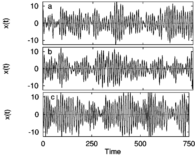
FIG. 1. Realizations of the processes investigated. (a) AR2 process satisfying the null hypothesis. (b) Amplitude modulated process with modulation depth of 0.3. (c) Period modulated process, relative amplitude of modulation is 15%.
