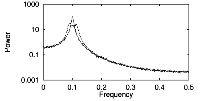
FIG. 2. Estimated spectra of the processes shown in Fig. 1. The spectra corresponding to Figs. 1(a) and 1(b) are not distinguishable (solid line). Period modulated process (dashed line).
