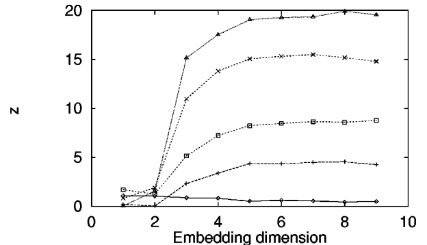
FIG. 4. Results of the simulation study for the period modulated process. Shown is z in dependence on the embedding dimension for different degrees \mathcal{M}_T of violation ( \diamond = 0 , + = 1, \square = 1.5, \times = 2, \triangle = 3).
