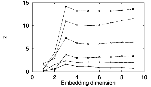
FIG. 3. Results of the simulation study for the amplitude modulated process. Shown is z in dependence on the embedding dimension for different degrees \mathcal{M}_{\text{amp}} of violation ( \diamond = 0 , + = 0.1, \square = 0.2, \times = 0.3, \triangle = 0.4, * = 0.5).
